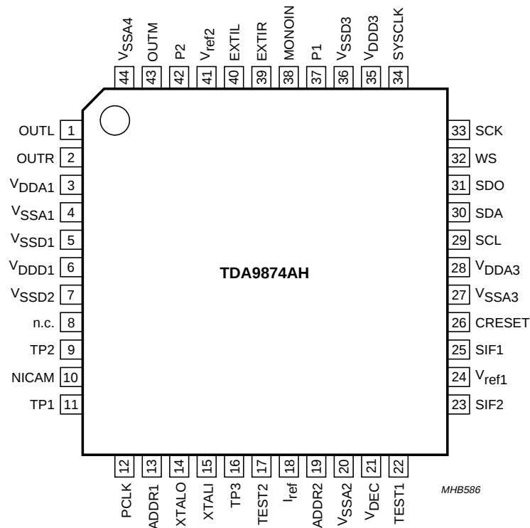
Fig.3 Pin configuration (QFP44).
